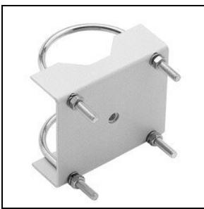
14012294 Steel 'U' bolt clamp for Ø 60-80 mm poles painted aluminium grey GR-94 / Metallic grey
